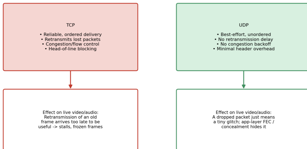
Figure 1.1 — Why the choice of transport protocol changes the user-visible effect of packet loss.
