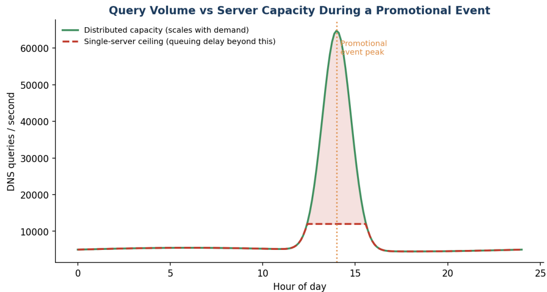
Figure 3.3 — A single server's fixed capacity ceiling is exactly what turns a traffic spike into user-visible delay.
